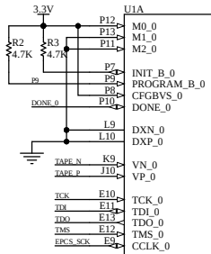
XC7A15T-1CSG324C
