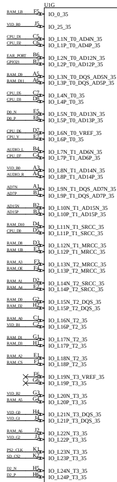
XC7A15T-1CSG324C
